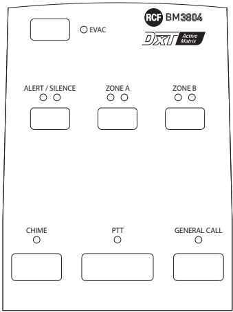
Front panel
